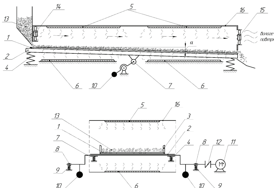
Fig. 3. Scheme of the conveyor tray infrared dryer: 1 – tray; 2 – spring-loaded platform; 3 – flanges; 4, 9 – elastic elements; 5, 6 – infrared emitters; 7 – eccentric shaft; 8 – support units of the vibrator; 10 – counterweights; 11 – electric motor; 12 – elastic coupling; 13 – grain products; 14, 15 – fans; 16 – working chamber of the dryer; \alpha – angle of the vibrating tray
